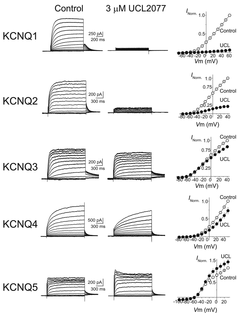
Fig. 2. UCL2077 modulates KCNQ channels in a subtype-selective manner. Left and middle, representative current traces at different membrane potentials from heterologous cells expressing KCNQ1, KCNQ2, KCNQ3, KCNQ4, or KCNQ5 before (left) and after (middle) application of 3 \mu\text{M} UCL2077. Right, current-to-voltage relationships for each KCNQ subunit are shown. Normalized current values were plotted against test potentials before ( \circ ) and after ( \bullet ) the addition of 3 \mu\text{M} UCL2077. For these experiments, KCNQ currents were measured at various test potentials elicited by a short (1–1.5 s) depolarization from -70 mV and were followed by a return step to -55 mV. Test potentials were at 10-mV increments with the following ranges: KCNQ1, -70 to +60 mV; KCNQ2 and KCNQ3, -80 to +40 mV; KCNQ4, -80 to +50 mV, and KCNQ5, -100 to +30 mV.
